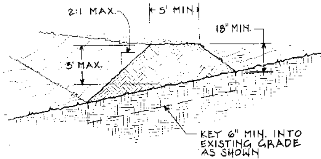
Figure 11. Temporary Containment Berm
