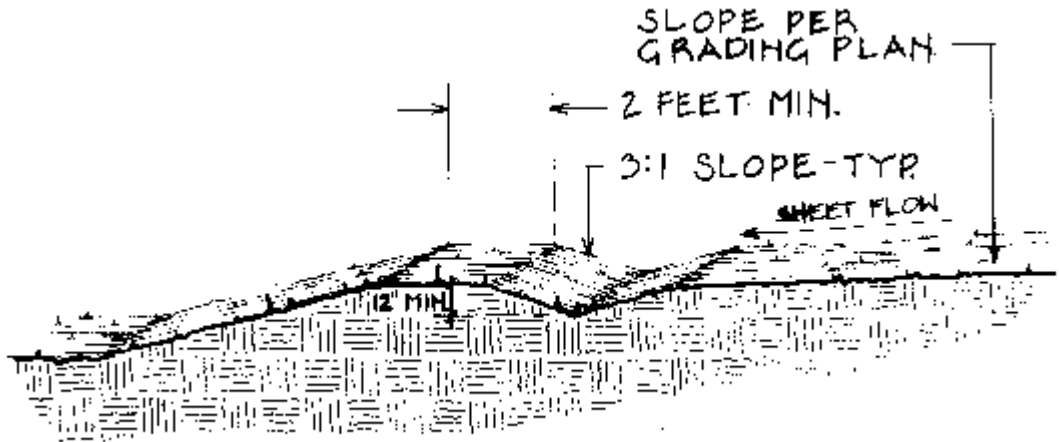
Figure 1. Diversion Swale
