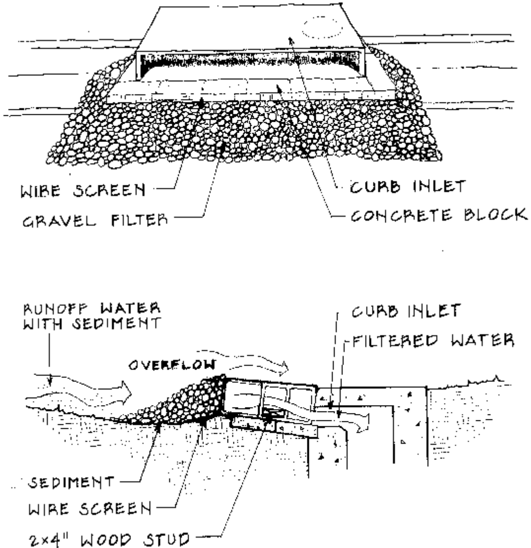
Figure 19. Block and Gravel Curb Inlet Sediment Filter
